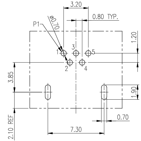
RECOMMEND PC BOARD LAYOUT TOLERANCE: ±0.05 mm
