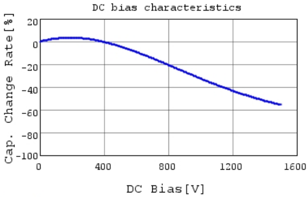
DE1E3RA102MA4BQ01F C-DC bias capchange, 20.0
