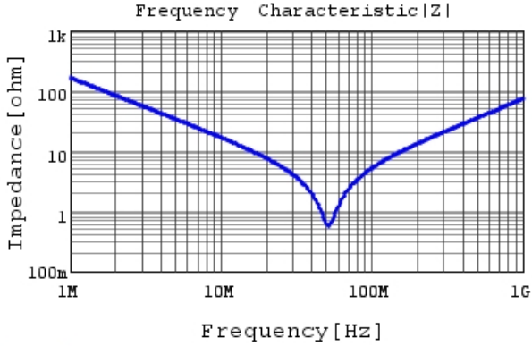
DE1E3RA102MA4BQ01F |Z| DC0V, 20degC
