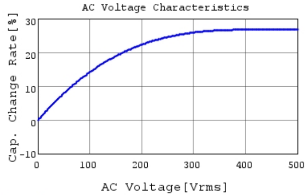
DE1E3RA102MA4BQ01F C-AC Voltage capchange, I
