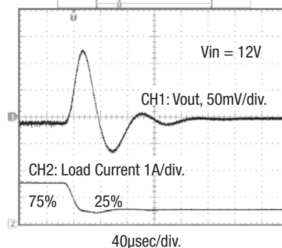
78SR-5/2 75% to 25% Load Step
