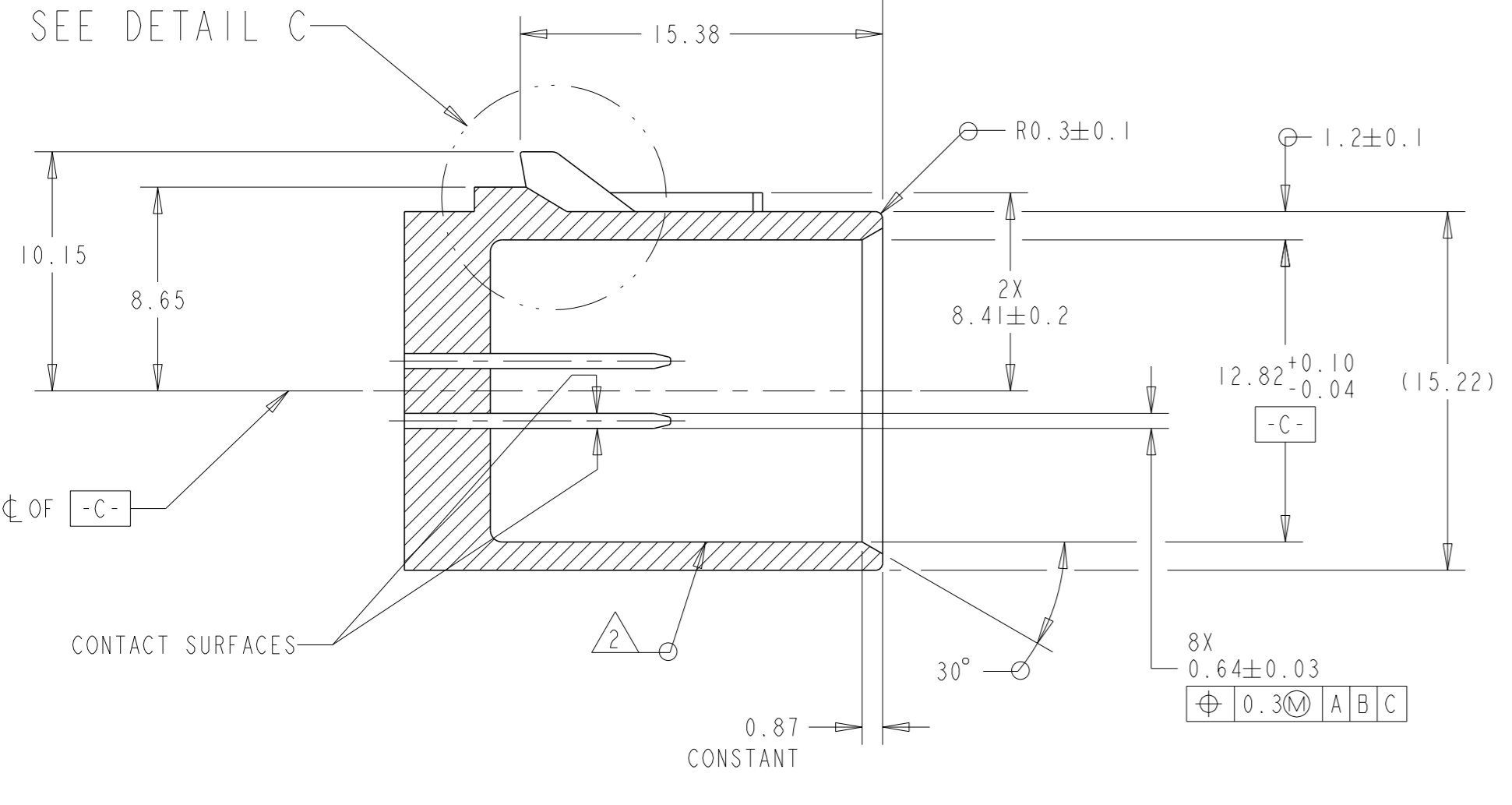
SECTION B-B
