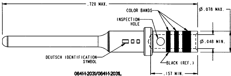
0641-2031/0641-2031L SIZE 20
