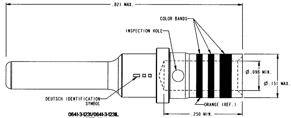
0641-3-1231/0641-3-1231L SIZE 12
