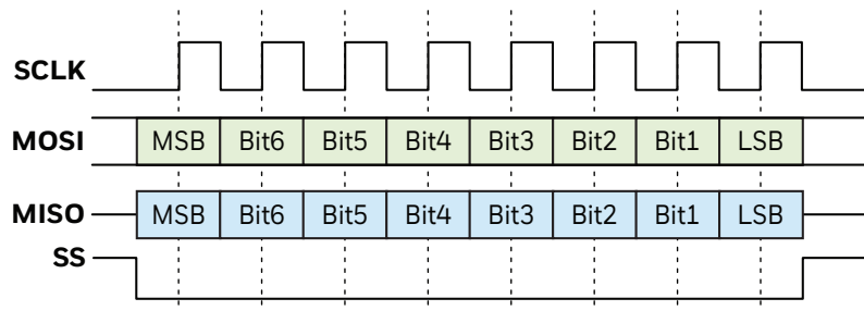
FIGURE 12. EXAMPLE OF 1 BYTE SPI DATA TRANSFER
