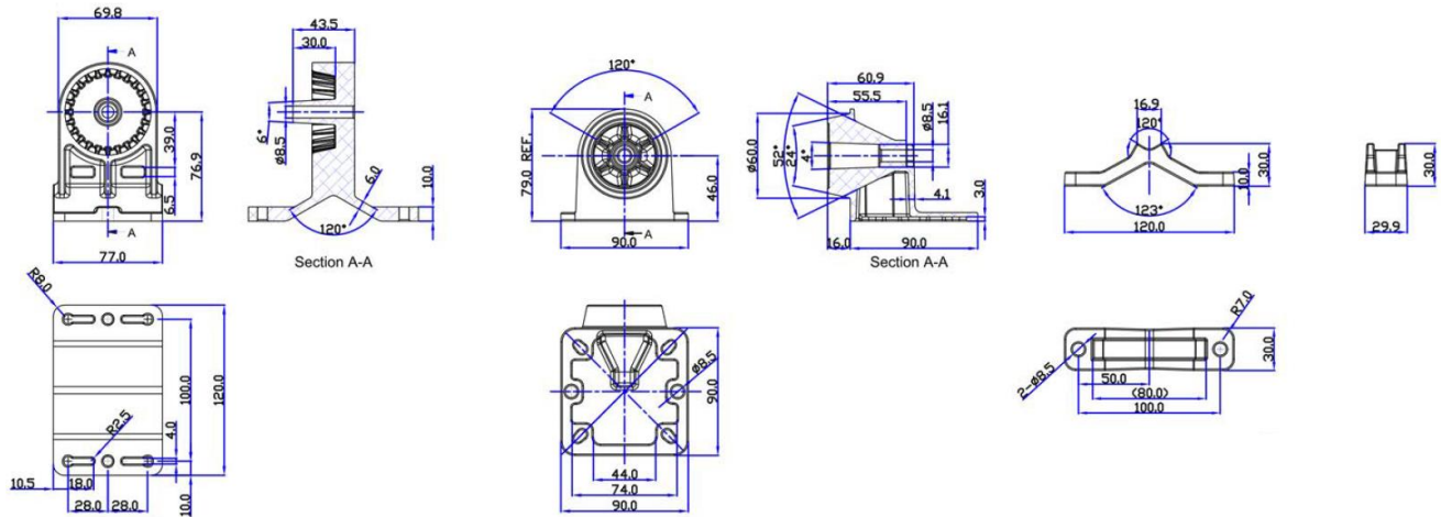
Figure 57: Pole mount dimensions
