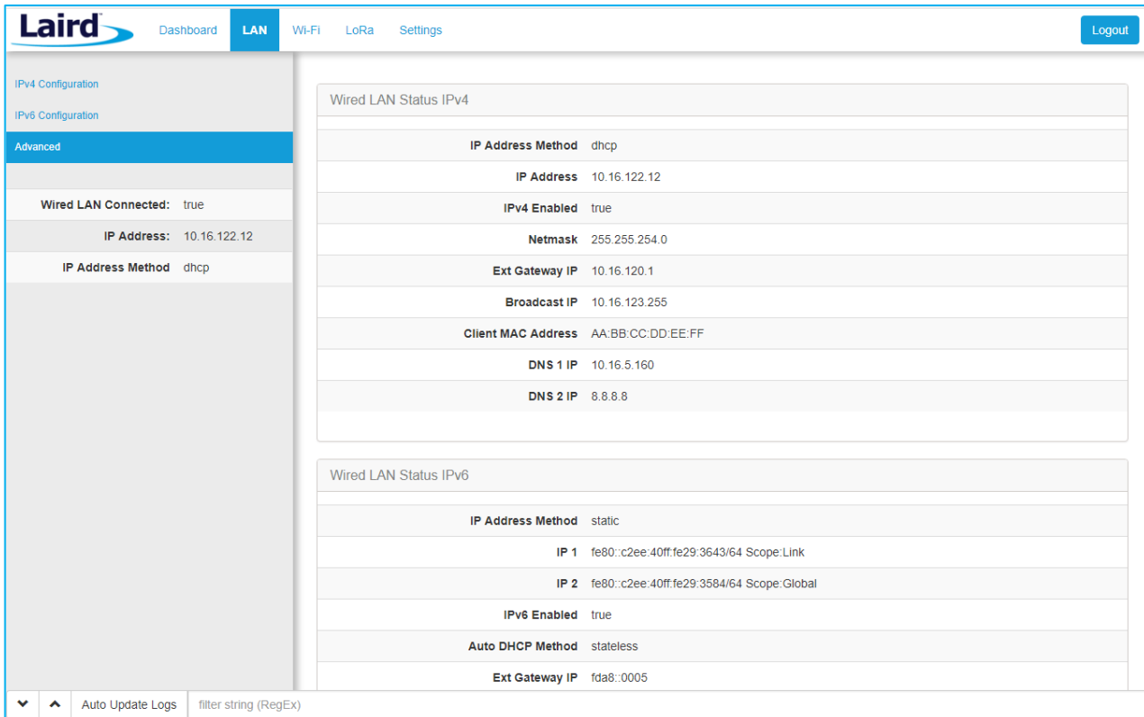
Figure 12: Advanced view
