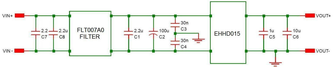
Figure 29. EMC Considerations
