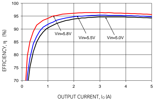
Figure 7. Converter Efficiency versus Output Current ( V_{out} = 4.0Vdc ).
