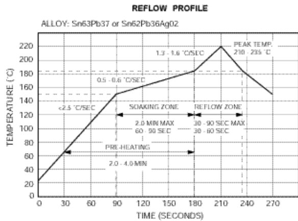
Figure 37. Reflow Profile.
