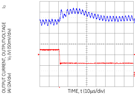
Figure 14. Transient Response to Dynamic Load Change from 100% of 50% full load ( V_o = 5.0\text{ Vdc} , C_{ext} = 2 \times 150\ \mu\text{F} Polymer Capacitors).
