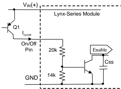
Figure 29. Remote On/Off Implementation.
