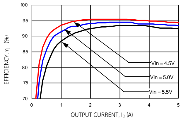
Figure 6. Converter Efficiency versus Output Current ( V_{out} = 3.3Vdc ).
