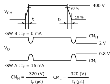
Fig. 13.1.6 Common-Mode Transient Immunity Test Circuit and Waveform
