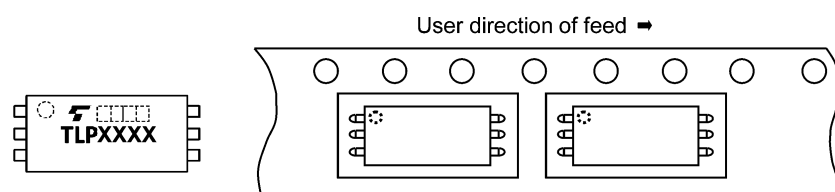
Fig. 18.3.1.1 Orientation of Device in Relation to Direction of Tape Movement
