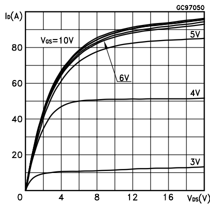
Figure 3. Output characteristics
