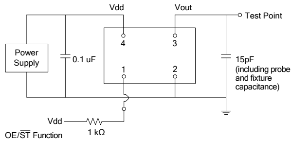
Figure 1. Test Circuit
