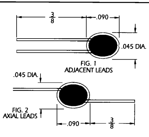
All illustration dimensions are in inches.
