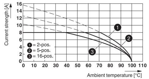
Type: MCVW 1,5/...-ST-3,81 with MC 1,5/...-G-3,81
