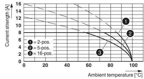
Type: IMC 1,5/...-G-3,81 with MC 1,5/...-G-3,81
