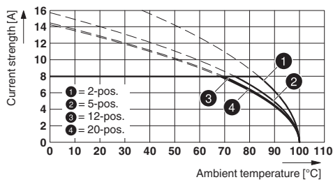
Type: FMC 1,5/...-ST-3,81 with MC 1,5/...-G-3,81
