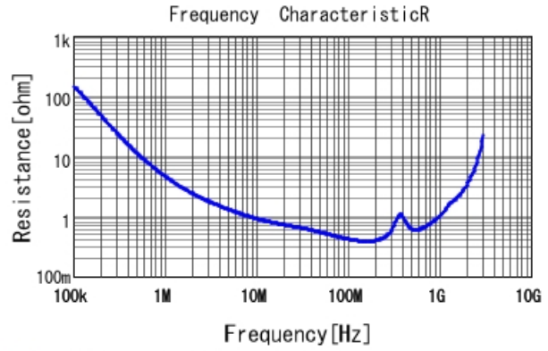
■ GA352QR7GF681KW01 R DCOV, 25degC
