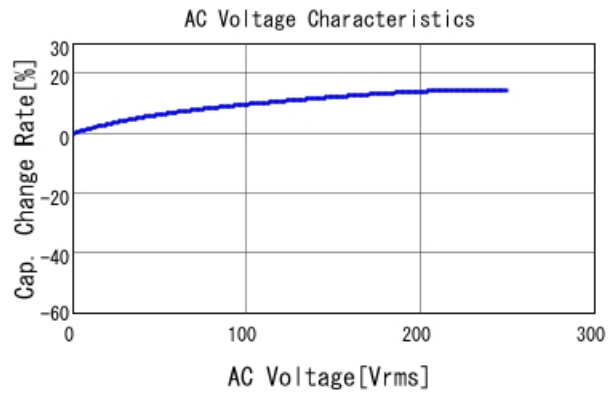
■ GA352QR7GF681KW01 C-AC Voltage capchange, DCOV, 25.0d
