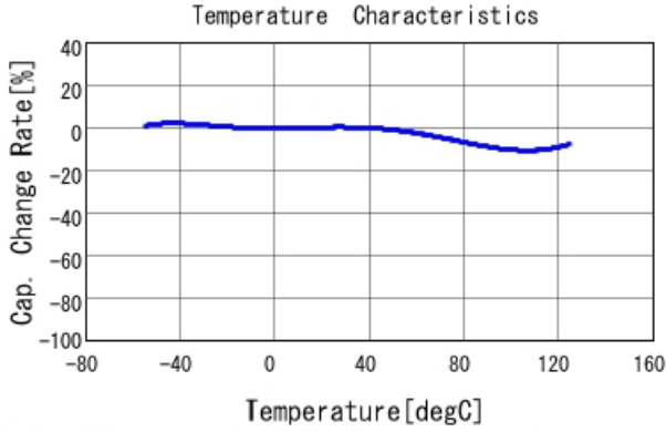
■ GA352QR7GF681KW01 C-Temp. capchange, DCOV, AC1Vrms
