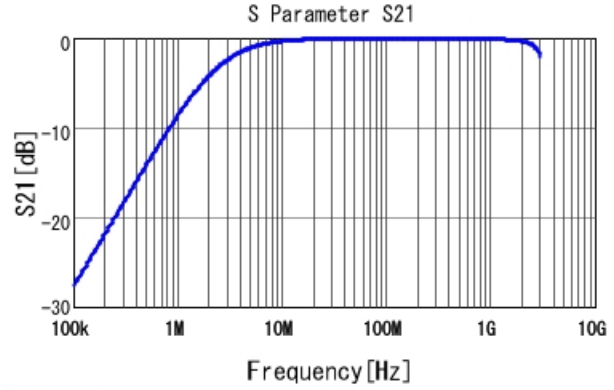
■ GA352QR7GF681KW01 S21 DCOV, 25degC
