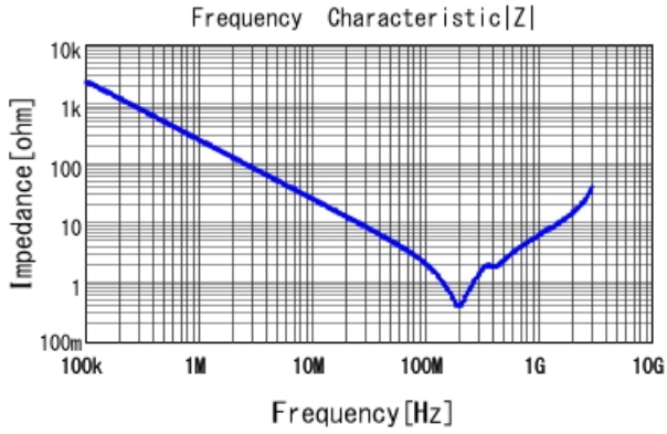
■ GA352QR7GF681KW01 |Z| DCOV, 25degC
