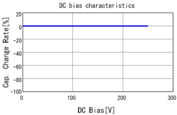
■ GA352QR7GF681KW01 C-DC bias capchange, 25.0degC, AC1V
