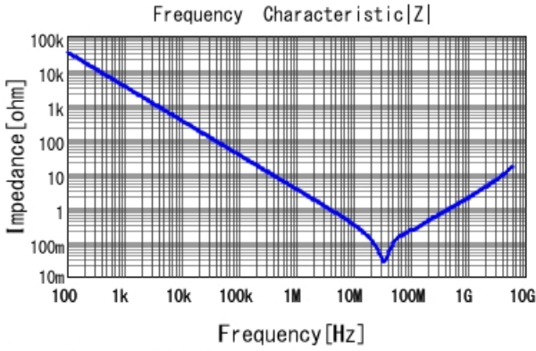
GCM188R71H473KA55 |Z| DCOV, 25degC
