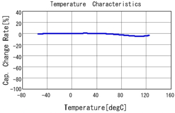
GCM188R71H473KA55 C-Temp. capchange, DC0.0V, AC1.C
