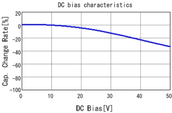
GCM188R71H473KA55 C-DC bias capchange, 25.0degC, A
