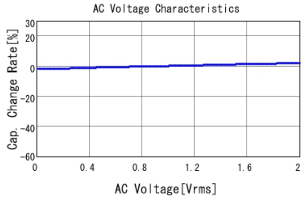
GCM188R71H473KA55 C-AC Voltage capchange, DCOV, 25
