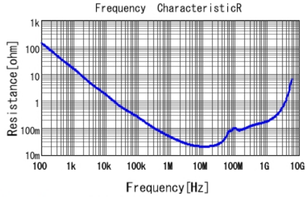
GCM188R71H473KA55 R DCOV, 25degC
