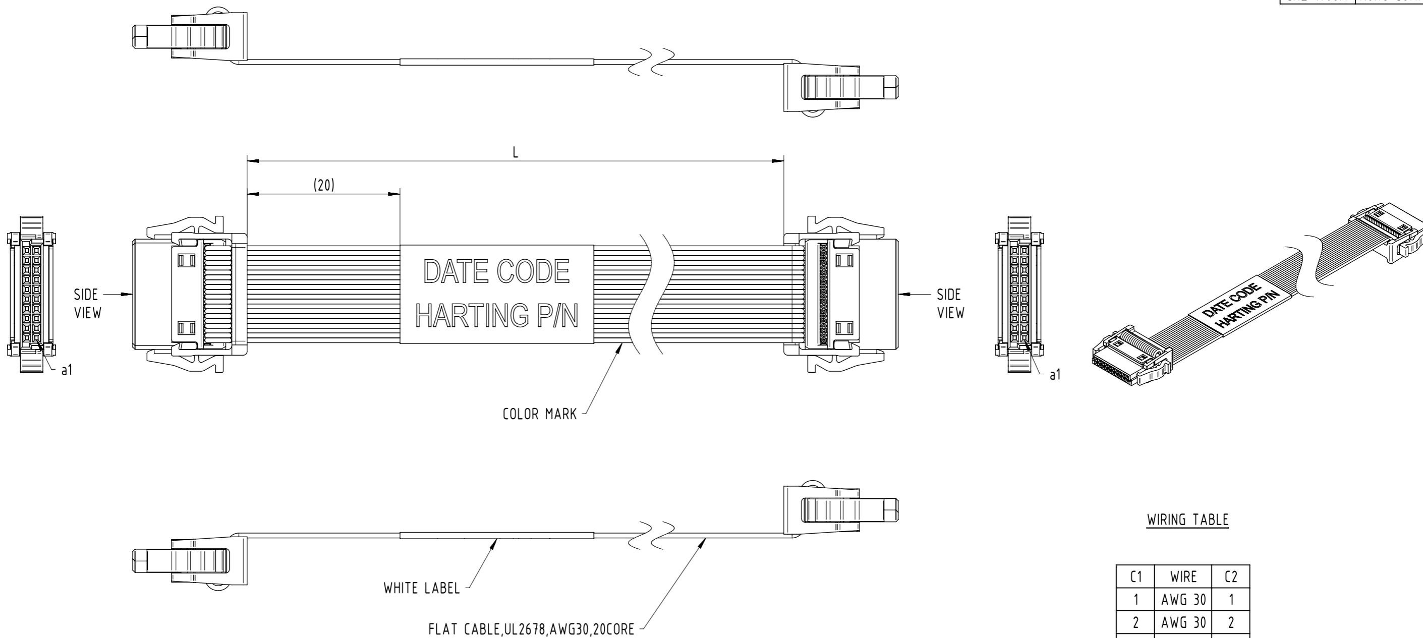
C1 HAR-FLEX 20 POLE FEMALE CONNECTOR WITH STRAIN RELIEF
