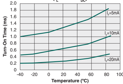
Typical Turn-On Time vs. Temperature ( I_L=170mA_{DC} )
