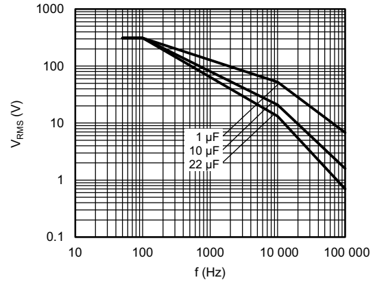
Maximum RMS voltage as function of frequency T_{amb} \leq 85^\circ\text{C} ; U_n = 310\text{ V}_{AC}
