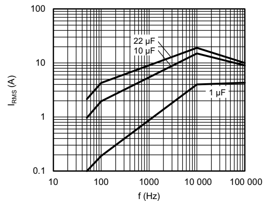
Maximum RMS current as function of frequency T_{amb} \leq 85^\circ\text{C} ; U_n = 310\text{ V}_{AC}
