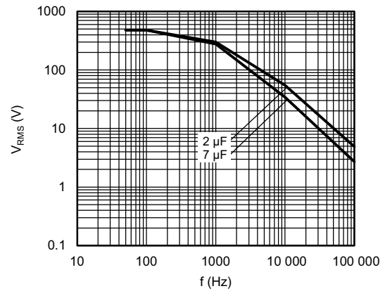
Maximum RMS voltage as function of frequency T_{amb} \leq 85^\circ\text{C} ; U_n = 480\text{ V}_{AC}
