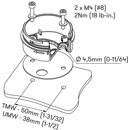
TMW, UMW - UL Type 4/4X/13
