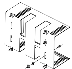
Fastening lugs (cards mounted vertically)
