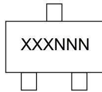
3-lead SOT-23
