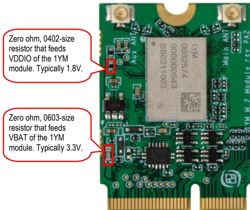
Figure 7 – Current Measurement
