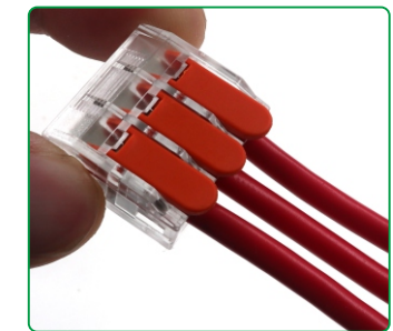
4) Installation is complete
