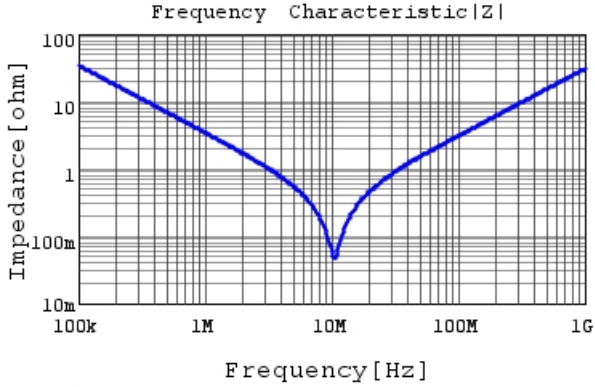
RDER72A473K1S1H03A |Z| DC0V, 25degC
