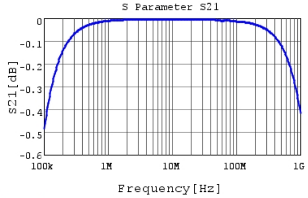
RDER72A473K1S1H03A S21 DC0V, 25degC
