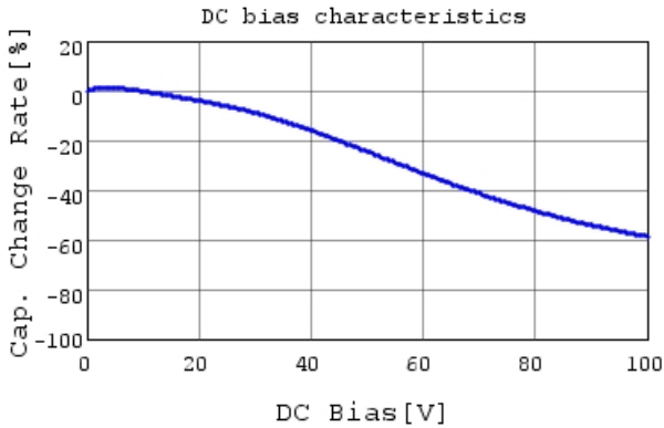
RDER72A473K1S1H03A C-DC bias capchange, 25.0
