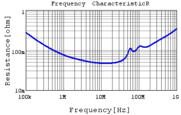
RDER72A473K1S1H03A R DC0V, 25degC
