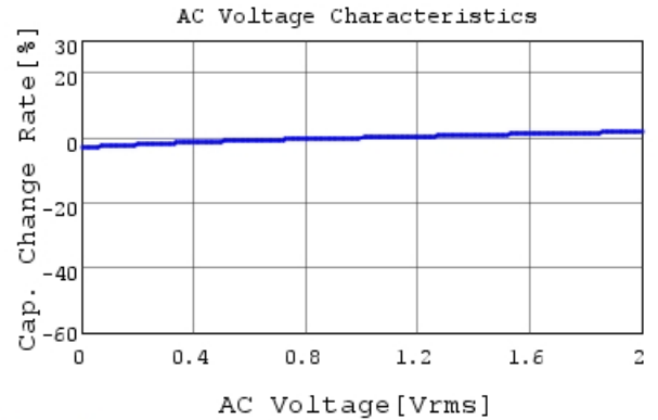
RDER72A473K1S1H03A C-AC Voltage capchange, I
