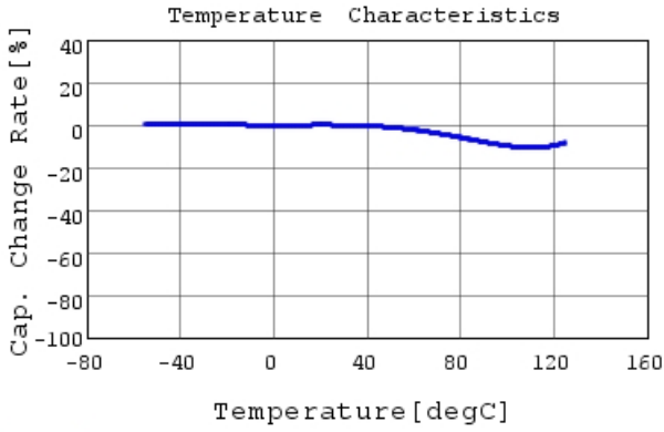
RDER72A473K1S1H03A C-Temp. capchange, DC0.0V
