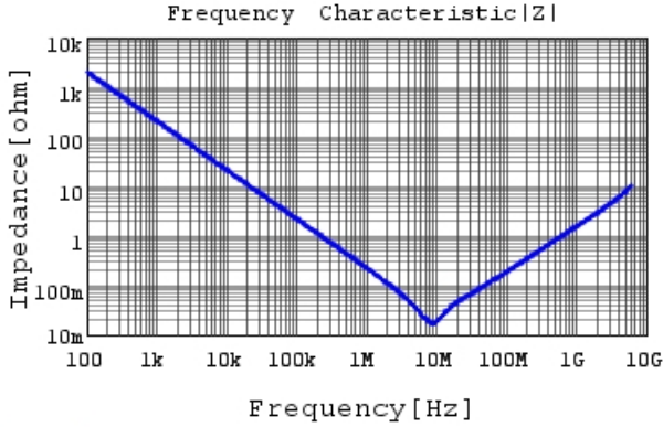
GCM155C71A105KE38 |Z| DC0V, 25degC
