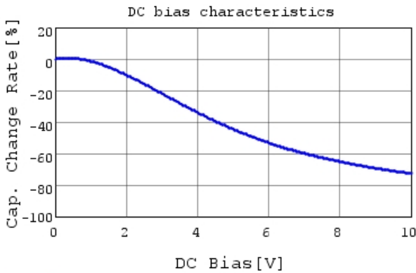
GCM155C71A105KE38 C-DC bias capchange, 25.0c
