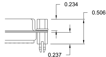
91 ..... 0.237" BOARD SIDE
