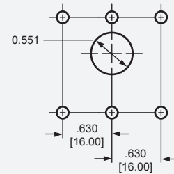
Three Pole
