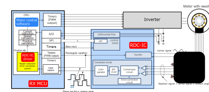
Motor control configuration
