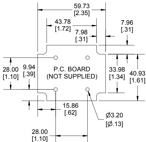
INSIDE TOP
