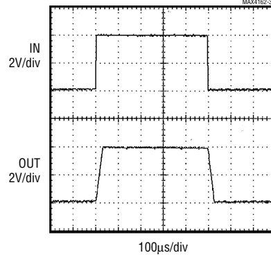
NONINVERTING LARGE-SIGNAL PULSE RESPONSE ( V_{DD} = 5V , C_L = 0 )
