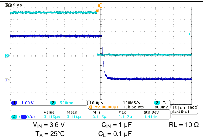
Figure 21. Turn-Off Response
