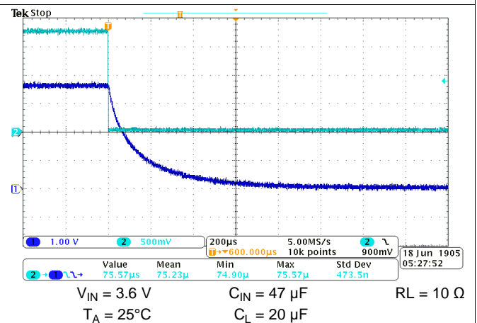
Figure 23. Turn-Off Response
