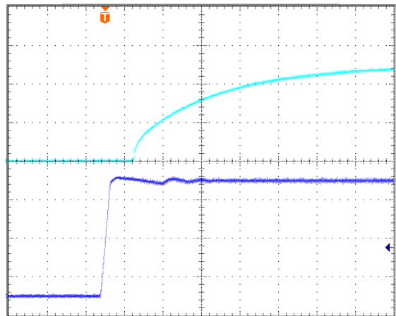
Turn-on transient at full load current (10 ms/div). Top Trace: Vout; 2V/div; Bottom Trace: input voltage: 8V/div.
