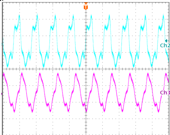
Output voltage ripple at nominal input voltage and max load current Top trace +15V, 10mV/div, Bottom trace -15V, 20mV/div, 2 \mu s/div.
