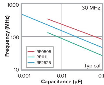
SERIES RESONANCE vs. CAPACITANCE
