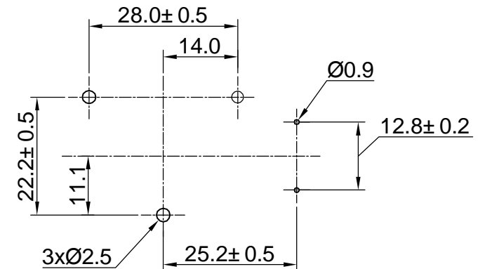
PCB/MOUNTING LAYOUT
