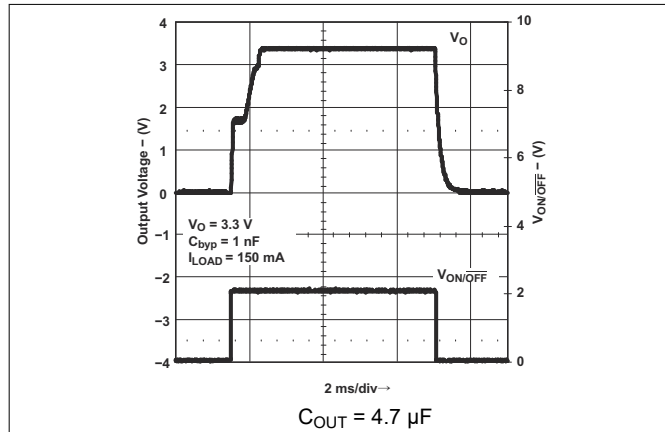
Figure 8-21. Turn-On Time for Legacy Chip
