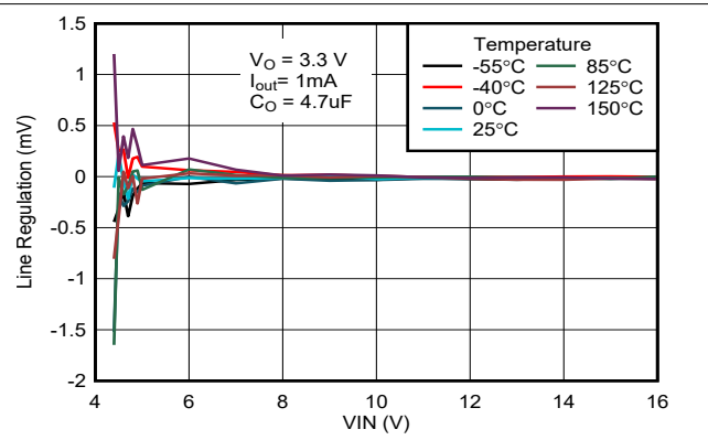
Figure 6-8. Output Regulation vs Input Voltage for New Chip
