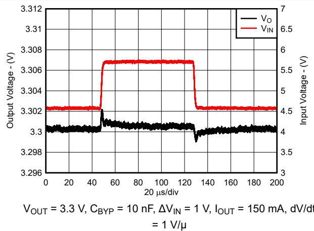
Figure 8-12. Line Transient Response for New Chip
