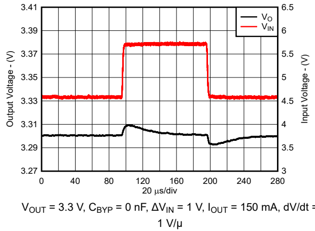
Figure 8-10. Line Transient Response for New Chip
