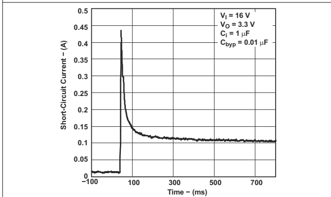
Figure 6-9. Short-Circuit Current vs Time for Legacy Chip
