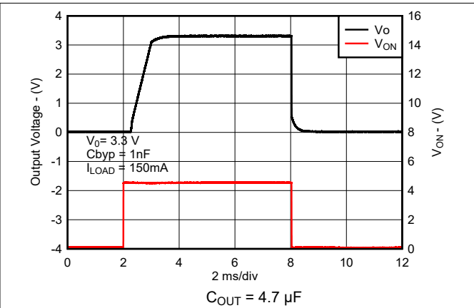
Figure 8-22. Turn-On Time for New Chip
