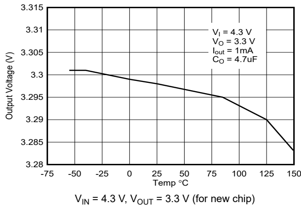
Figure 6-3. Output Voltage vs Temperature for New Chip
