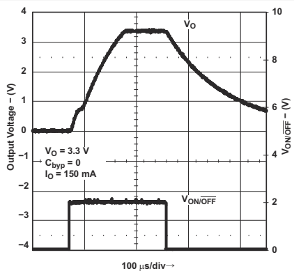
Figure 8-17. Turn-On Time for Legacy Chip
