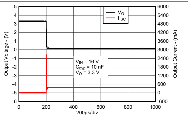
Figure 6-10. Short-Circuit Current vs Time for New Chip
