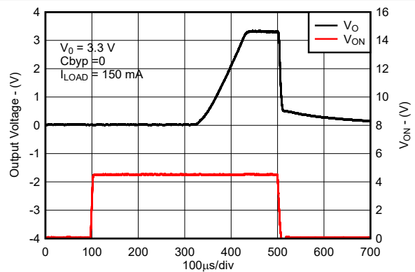
Figure 8-18. Turn-On Time for New Chip
