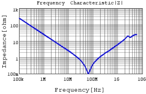
GRM31BR72J682KW01 |Z| DCOV, 25degC
