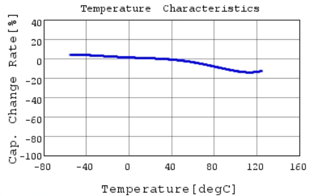
GRM31BR72J682KW01 C-Temp. capchange, DCOV, 1
