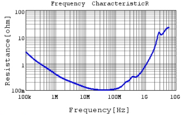
GRM31BR72J682KW01 R DCOV, 25degC
