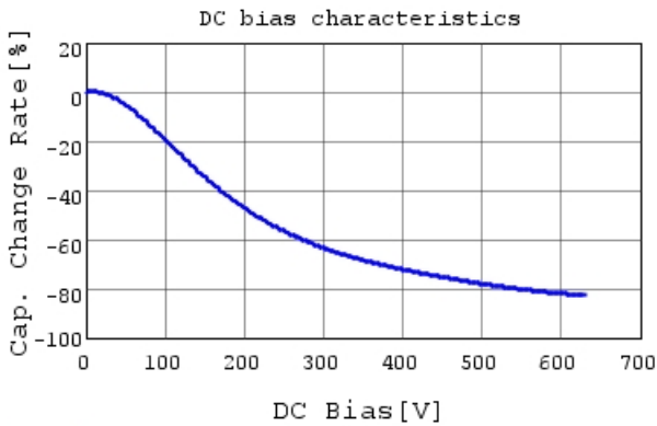
GRM31BR72J682KW01 C-DC bias capchange, 25.0c
