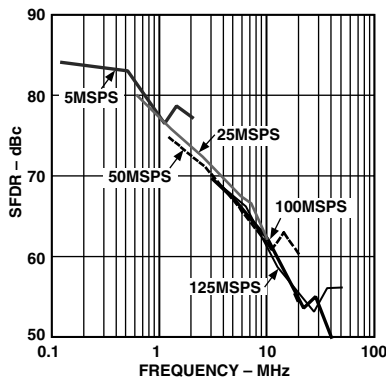
Figure 21. SFDR vs. f_{OUT} @ 0 dBFS
