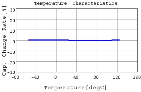
GRM1885C1H562JA01 C-Temp. capchange, DCOV, 1
