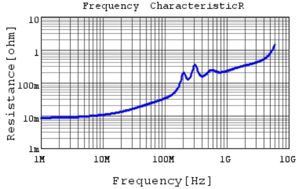
GRM1885C1H562JA01 R DCOV, 25degC
