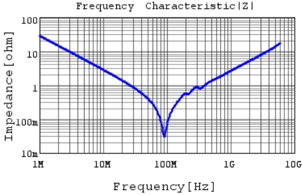
GRM1885C1H562JA01 |Z| DCOV, 25degC
