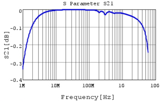
GRM1885C1H562JA01 S21 DCOV, 25degC
