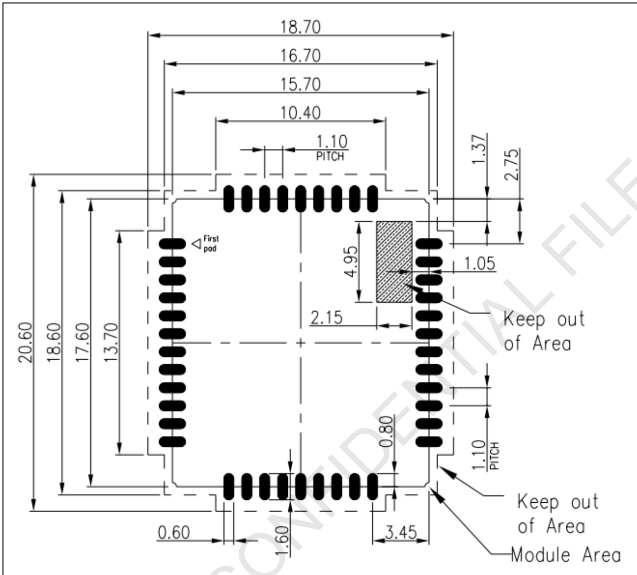
Figure 4: Recommended PCB footprint outline (Unit: mm)
