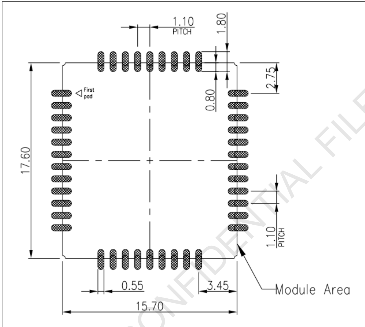
Figure 5: Recommended SMT stencil footprint outline (Unit: mm)
