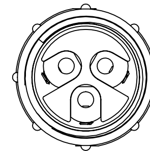
WIRING END VIEW (3 POS) WITHOUT REAR END HARDWARE
