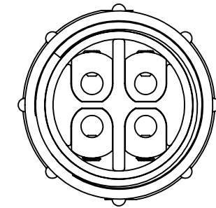
WIRING END VIEW (4 POS) WITHOUT REAR END HARDWARE
