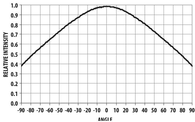
Figure 5: Radiation Pattern
