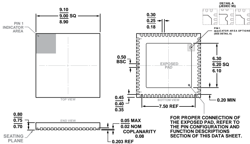
Figure 33. 64-Lead Lead Frame Chip Scale Package [LFCS] 9 mm x 9 mm Body and 0.75 mm Package Height (CP-64-17) Dimensions shown in millimeters
