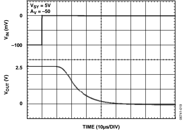
Figure 22. AD8538 Negative Overload Recovery
