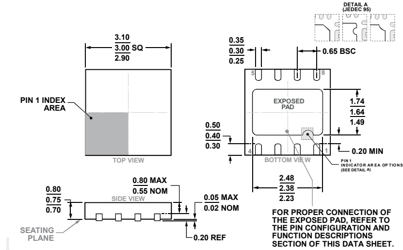
Figure 65. 8-Lead Lead Frame Chip Scale Package [LFCSP] 3 mm x 3 mm Body and 0.75 mm Package Height, Dual Lead (CP-8-3)
