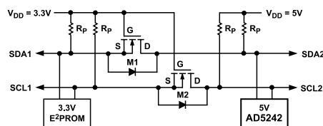
Figure 33. Level-Shift for Different Voltage Devices Operation
