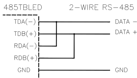
Figure 3. 2-Wire RS-485
