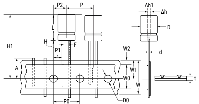
Fig. 4 (Diameter for \Phi 10 ) 10 mm EA
