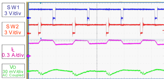
Figure 12. Buck-boost region operation @ I_O = 500\text{ mA}
