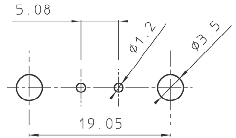
DRILLING HOLE PATTERN
